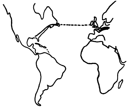
FIG. 475.—The interrupted system of the Appalachian Mountains common to western Europe and eastern North America (after Arldt).
